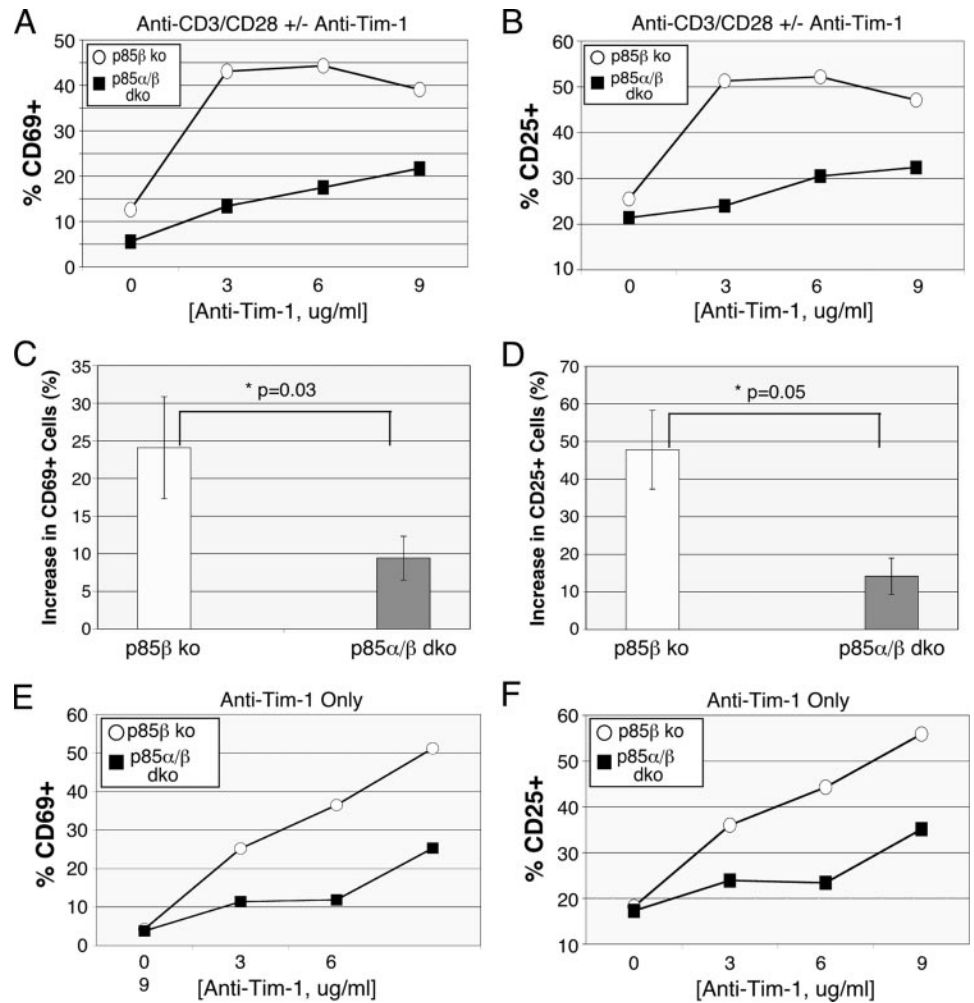
FIGURE 7. p85 is required for Tim-1-mediated CD69 and CD25 up-regulation. Purified CD4 + T cells from p85 \beta - or p85 \alpha/\beta -deficient mice were stimulated in vitro with anti-CD3/CD28 Abs (20 ng/ml and 0.5 \mu g/ml, respectively) and the indicated concentrations of Tim-1 Ab (A–D) or with anti-Tim-1 Ab alone (E and F). Cells were harvested and stained for CD69 (A, C, and E) or CD25 (B, D, and F) expression, and analyzed by flow cytometry. Results in A and B, and E and F, are single experiments, representative of three, or two, separate experiments, respectively. C and D, Effects of Tim-1 costimulation ( \pm SD) averaged over those experiments, with p values indicated.
