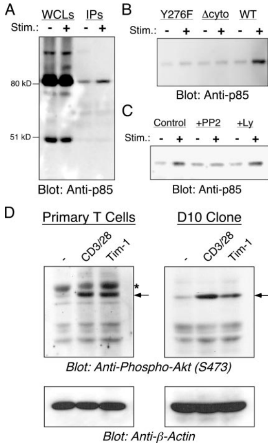
FIGURE 3. Recruitment and activation of PI3K by Tim-1. A , Jurkat T cells expressing Flag-Tim-1 were stimulated as indicated, lysed, and immunoprecipitated with anti-Flag. Whole cell lysates (WCLs) and IPs were separated by SDS-PAGE and Western blotted for p85 \alpha/\beta . B , Jurkat T cells expressing the indicated wild-type or mutant Flag-Tim-1 constructs were stimulated and analyzed for p85 binding as described for A . C , Jurkat T cells expressing wild-type Flag-Tim-1 were stimulated in the presence of 10 \mu M PP2 (Src kinase inhibitor) or 10 \mu M Ly294002 (PI3K inhibitor) then analyzed for p85 binding as above. D , T cell blasts ( left panels ) or D10 Th2 T cells ( right panels ) were stimulated as indicated. Lysates were separated by SDS-PAGE and Western blotted with a rabbit mAb to phospho-Akt (S473; upper panels ). Blots were stripped and re-probed with a mouse mAb to \beta -actin ( lower panels ), to control for protein loading. The location of phospho-Akt is indicated by the arrows, whereas the star indicates a nonspecific band that is only observed in primary T cells. Results in each part are representative of three experiments.
