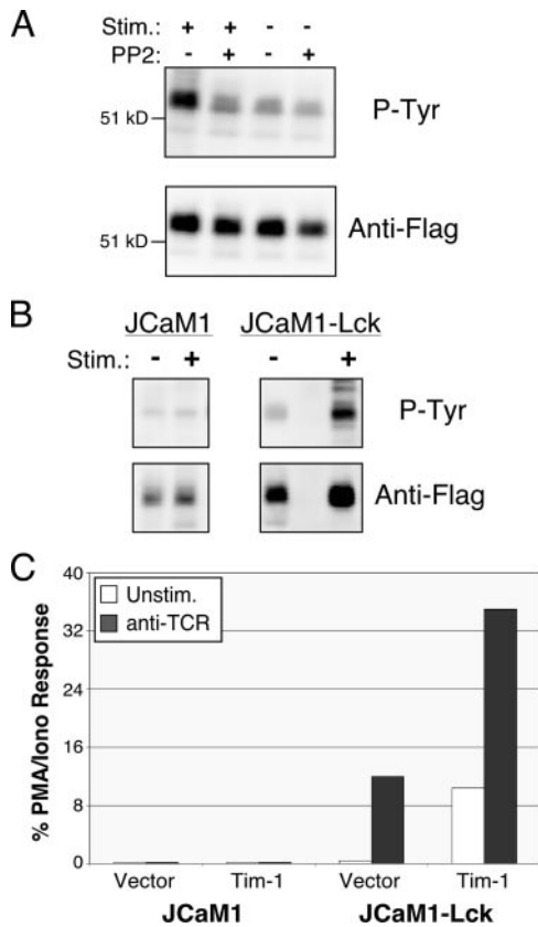
FIGURE 1. Role of Lck in Tim-1 tyrosine phosphorylation and function. A , Jurkat T cells expressing Flag-Tim-1 were stimulated as indicated, with or without the Src kinase inhibitor PP2. Anti-Flag immunoprecipitates were separated by SDS-PAGE and Western blotted with anti-Flag (lower panel), then stripped and re-probed with anti-phosphotyrosine Ab 4G10 (P-Tyr; upper panel). B , Lck-deficient JCaM1 or Lck-reconstituted JCaM1 cells expressing Flag-Tim-1 were stimulated and analyzed as in A . C , JCaM1 or JCaM1-Lck cells were transfected with an NFAT/AP-1 luciferase reporter and either empty vector or Flag-Tim-1. Cells were stimulated the next day and luciferase activity was determined. Each experiment is representative of two ( A and B ) or three ( C ) that were performed. stim, Stimulated; and unstim, unstimulated.
