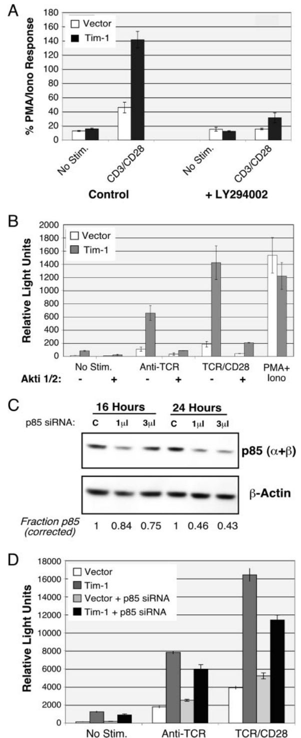
FIGURE 4. Role of the PI3K pathway in Tim-1 activation of NFAT/AP-1. T cells were transfected with an NFAT/AP-1 luciferase reporter and the indicated constructs, then stimulated the next day, as indicated, followed by determination of luciferase activity. A , Cells were stimulated in the presence or absence of the PI3K inhibitor LY294002. B , Cells were stimulated in the presence or absence of the Akt inhibitor Akti 1/2 (20 \mu M). C and D , T cells were transfected with an NFAT/AP-1 reporter, plus either empty vector or Flag-Tim-1, and the indicated amounts of short interfering RNA SmartPool oligos(dT) (Dharmacon) specific for p85 \alpha and p85 \beta . Twenty-four hours after transfection, cells were stimulated for 6 h, followed by determination of luciferase activity. Error bars indicate SD for triplicate points in a single experiment. Results shown in each part are representative of three experiments.
