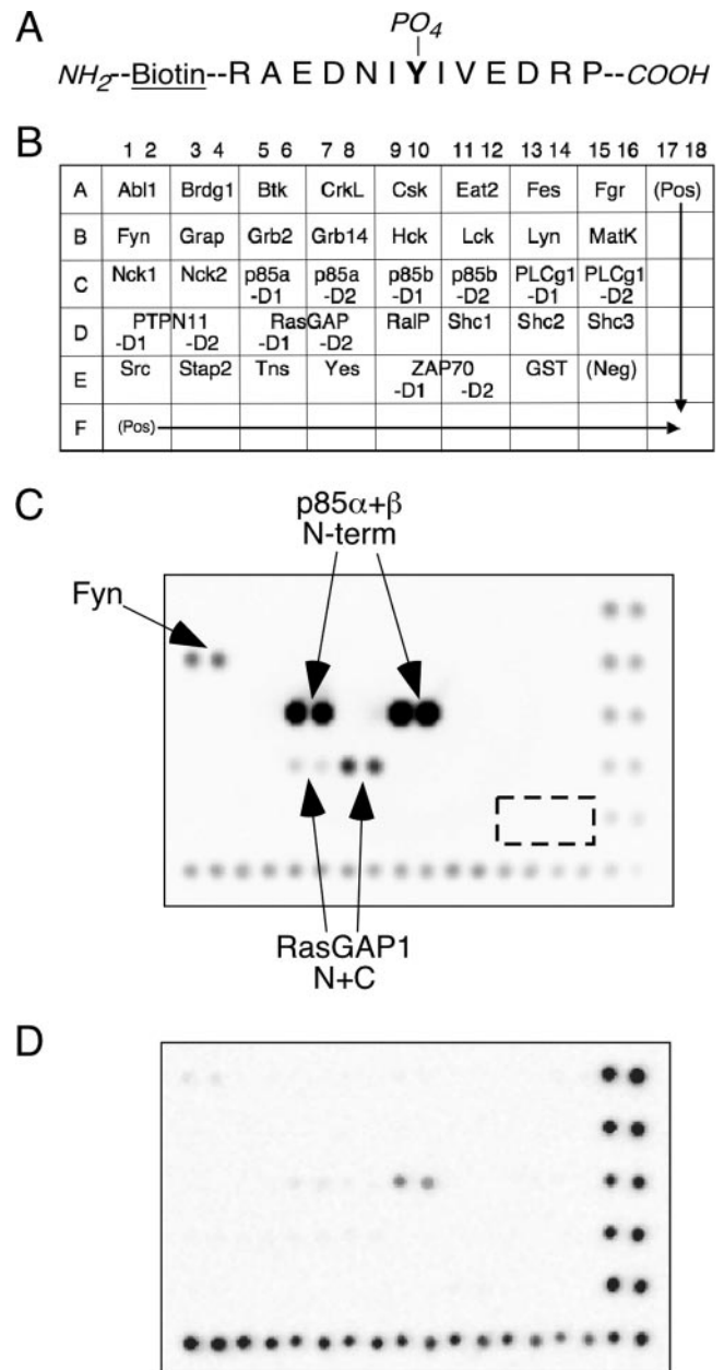
FIGURE 2. Specificity of SH2 domain binding to phosphorylated Y276 in the Tim-1 cytoplasmic tail. A , Sequence of the peptide, and modifications, used to determine the SH2 specificity of phospho-Y276. B , Layout of the SH2 domain array. SH2 domains are present as duplicate spots. For proteins with more than one SH2 domain, "D1" indicates the more N-terminal SH2. C , Results of the SH2 domain array screen, using the peptide illustrated in A . The dashed box indicates the location of negative control spots; the bottom and right edge contain positive control spots. These results are representative of those obtained in four separate experiments, using two different lots of membrane. D , Competitive inhibition of Tim-1 peptide binding by the phosphotyrosine analog phenylphosphate. The blot shown is representative of two experiments.
