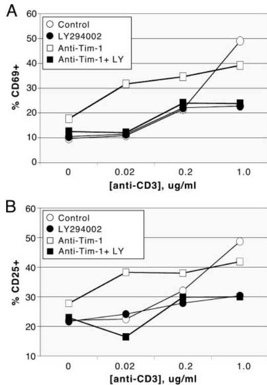
FIGURE 5. PI3K activity is required for up-regulation of early activation markers by endogenous Tim-1 on primary T cells. Purified CD4 + T cells from C57BL/6 spleen and lymph node were stimulated for 24 h with the indicated concentrations of anti-CD3 Ab (and a fixed concentration of anti-CD28 Ab, 0.5 \mu g/ml), with or without anti-Tim-1 Ab (6 \mu g/ml), in the presence or absence of PI3K inhibitor LY294002 (10 \mu M). Cells were stained with fluorescently labeled Abs to CD69 (A) or CD25 (B) and analyzed by flow cytometry. Results in each panel are representative of three experiments that were performed.
