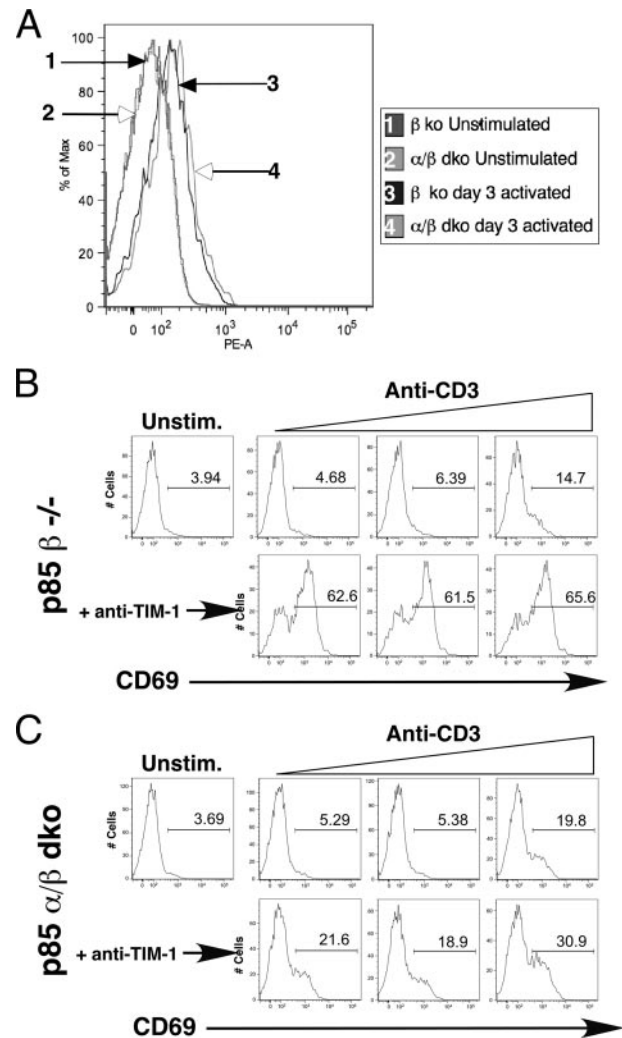
FIGURE 6. p85 is required for Tim-1-mediated costimulation of CD69 expression. A, Expression of Tim-1 on resting or activated CD4 + T cells from spleens of p85 \beta or p85 \alpha/\beta k.o. mice. Splenocytes from p85 \beta (B)- or p85 \alpha/\beta (C)-deficient mice were stimulated overnight with various concentrations anti-CD3 Ab (0.05, 0.2, and 1 \mu g/ml), along with a fixed concentration of anti-CD28 (1 \mu g/ml). Anti-Tim-1 Ab was also added to some cultures, at a concentration of 8 \mu g/ml. Cells were stained the next day for CD4 and CD69 and analyzed by flow cytometry. Results shown were gated on CD4 + cells.
